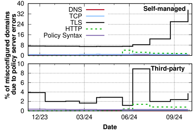
Figure 5: Percentage of MTA-STS enabled domains with misconfigured policy servers by error type and managing entity. In our latest snapshot, 9,588 (37.8%) self-managed and 1,393 (4.9%) third-party policy servers had misconfigurations. A spike on June 8, 2024, for third-party servers was due to a leading provider issuing self-signed certificates for 1,385 domains. Late spikes for self-managed domains were caused by Porkbun domains, as detailed in Figure 4.
