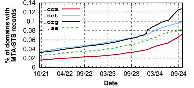
Figure 2: The deployment of MTA-STS records; 461 new domains related to the same organization under .org adopted MTA-STS in Jan 2, 2024 causing the notable spike.
