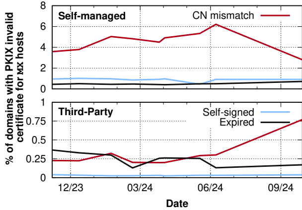
Figure 6: Percentage of MTA-STS enabled domains with PKIX invalid certificate for MX hosts; in our latest snapshot, 1,046 (4.4%) domains that self-manage their MX hosts and 397 (1%) domains that use email hosting services present PKIX-invalid certificates. 270 domains with self-hosted MX host fixed their Common Name mismatch error in our latest snapshot.
