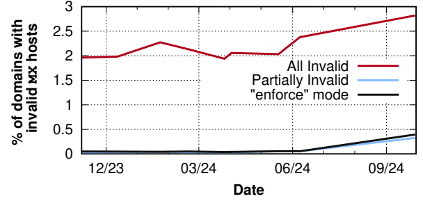
Figure 7: Percentage of MTA-STS enabled domains with all invalid, and partially invalid MX hosts. "enforce" mode presents domains with stricter policy and at least 1 invalid MX host; these are subject to potential email delivery failure from MTA-STS compliant senders and in our latest snapshot, we found 269 such domains.
