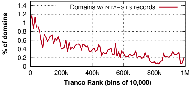
Figure 3: The percentages of domains publishing both MX and MTA-STS records as a function of website popularity based on Tranco 1M [33]; more popular websites are more inclined to deploy MTA-STS for their email services.
