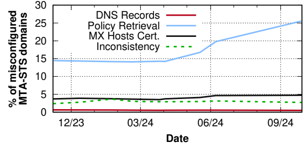
Figure 4: Percentage of MTA-STS enabled domains with errors in (1) MTA-STS records, (2) policy retrieval over HTTPS, (3) certificate of MX hosts, or (4) policy text where mx patterns of the policy file and MX records are inconsistent. Since August 2024, newly registered domains under Porkbun LLC [34] with invalid policy host certificates have increased policy server errors, affecting 7,237 domains in our latest snapshot.
